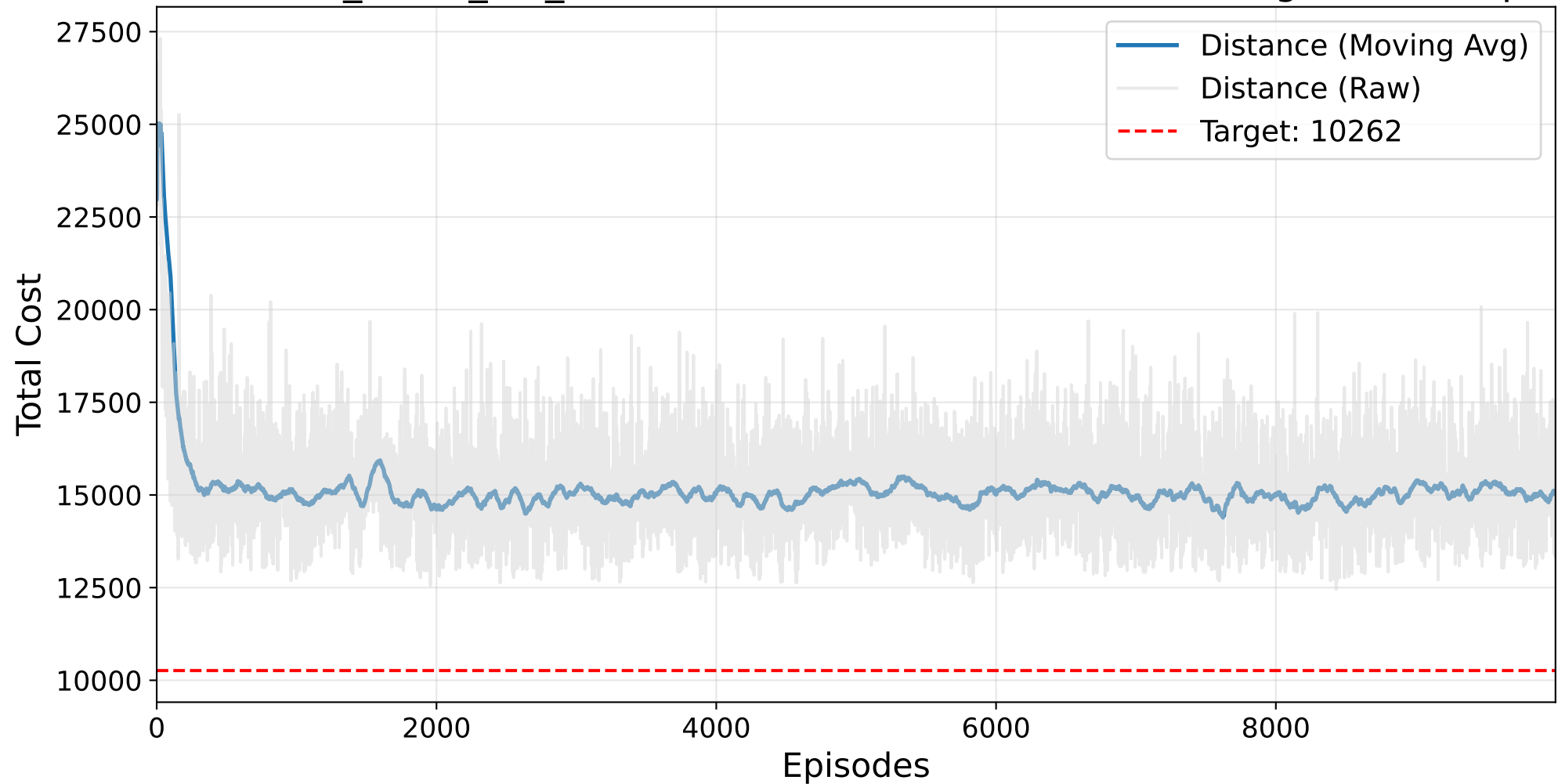
Final NO_MASK_NO_BAYESIAN Masked AutoRL-SOP Training - ft53.3.sop
